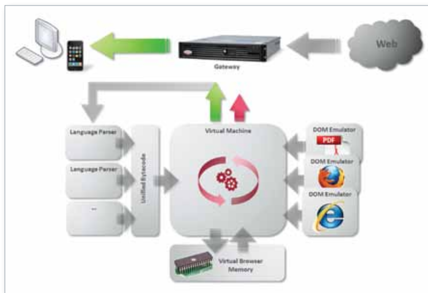
Figure 3. Browser emulation and behavioral profiling help to deliver protection from contemporary web attacks.
