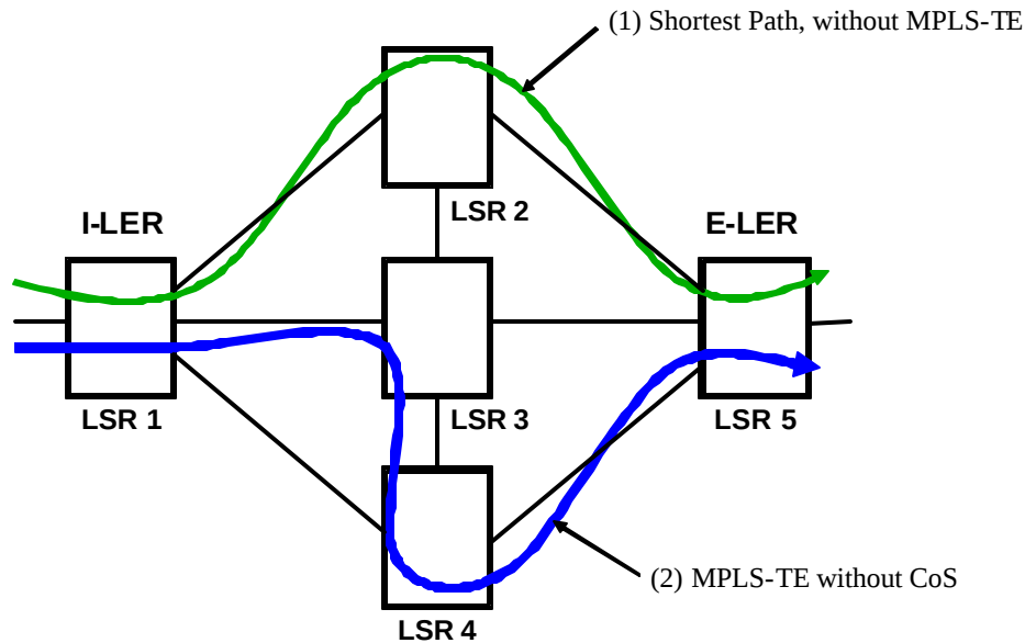
Figure 5. Packet flow in MPLS without DiffServ
