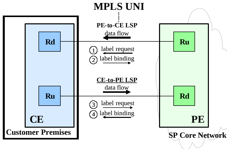
Figure 10. MPLS UNI
